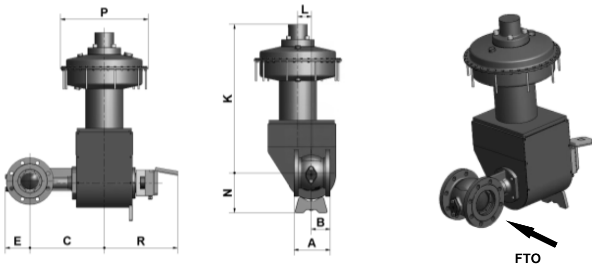
Fig. 24: Dimensions - Control valve Type 82.7-02 with MZ and MD · Assembly position B · FC (fail close)
