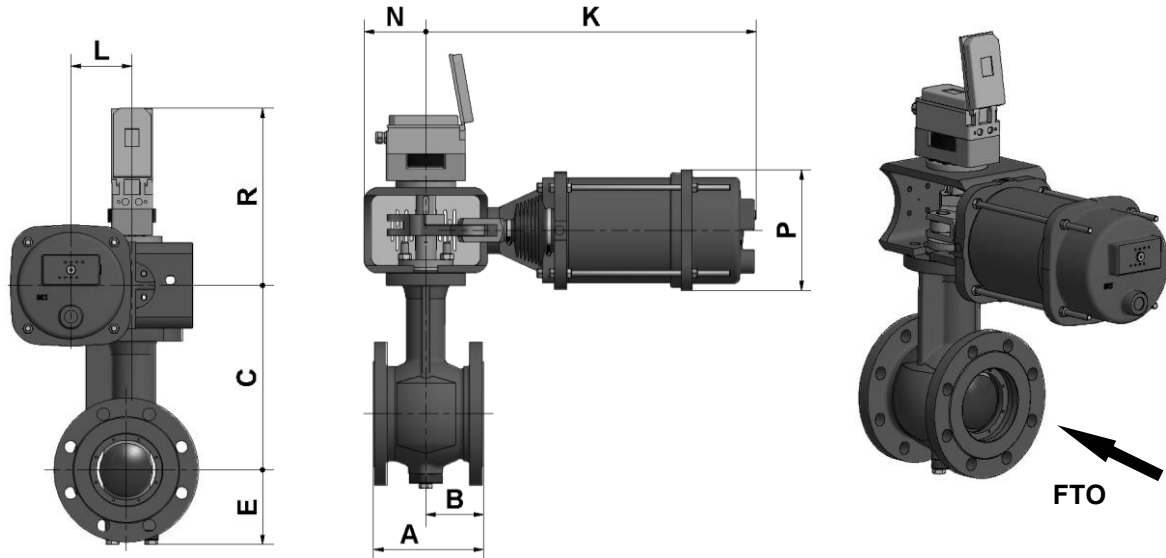
Fig. 23: Dimensions - Control valve Type 82.7-02/R · Assembly position A · FC (fail close)
