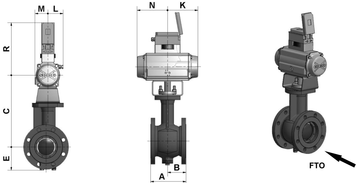
Fig. 22: Dimensions - Control valve Type 82.7-02/AT · Assembly position A/C · FO/FC
